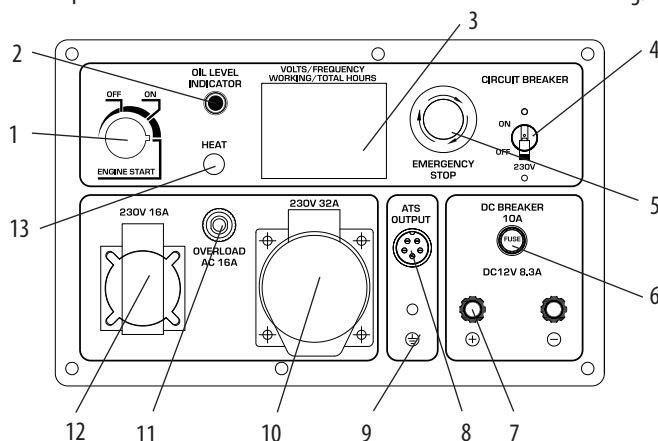
Control panel for model KS 11-2DE ATSR
