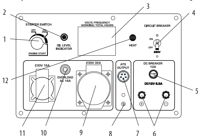
Control panel for model KS 9200HDE ATSR
